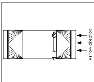
Airflow direction
