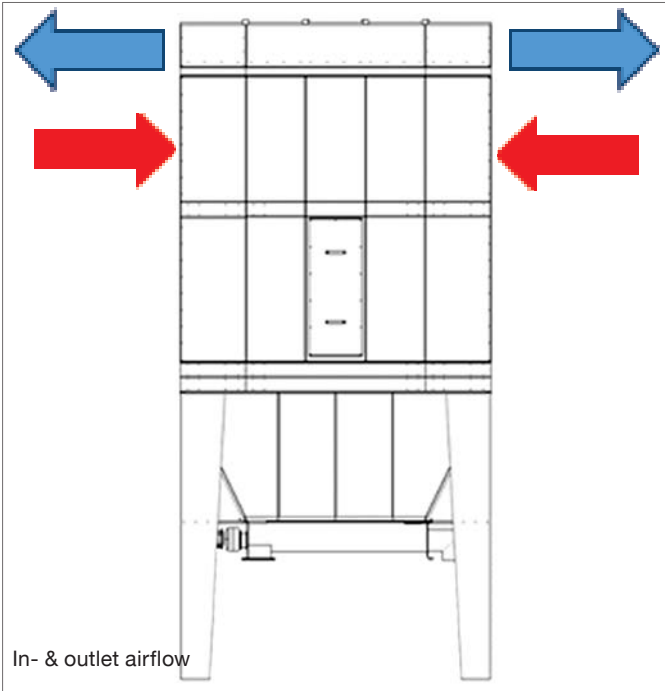
BERF 42 120 2500 1 T with screw and extraction fan in acoustic booth
