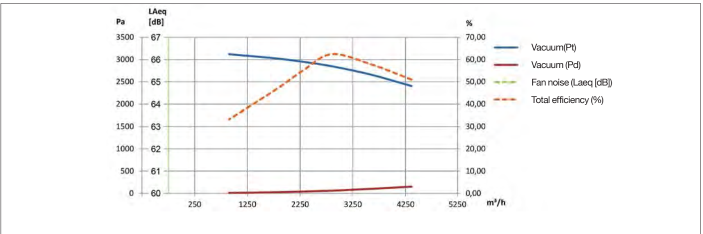
Fan type VR 5500 functioning curves at 2800 rpm
