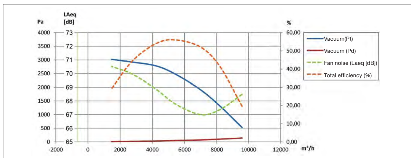
Fan type VE7500 functioning curves at 2800 rpm
