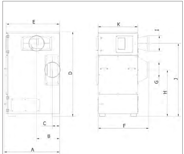
CFL filter unit without integrated fan
