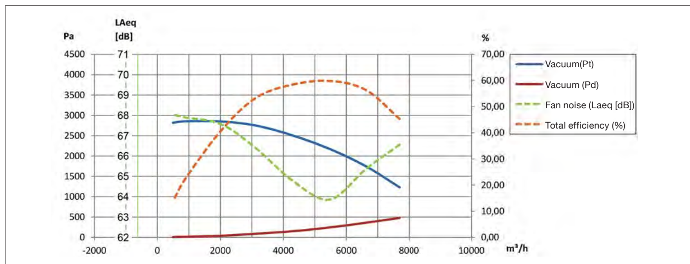
Fan type VE5500 functioning curves at 2800 rpm
