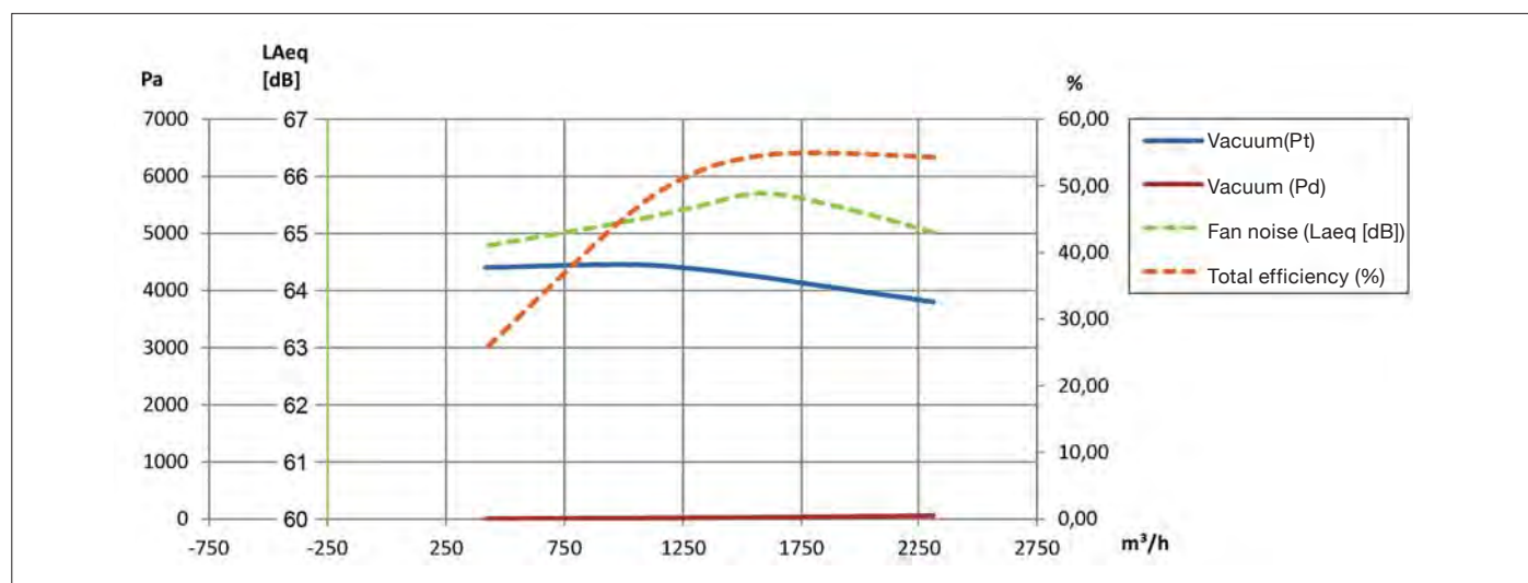
Fan type RVH35/2 functioning curves at 2800 rpm
